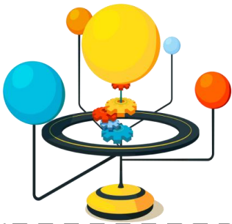
solar system
