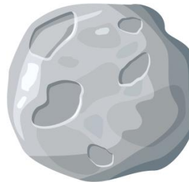
asteroid
